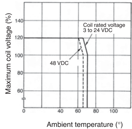
Ambient Temperature vs. Maximum Coil Voltage G5V-2
